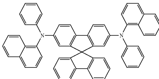
Spiro-NPB
